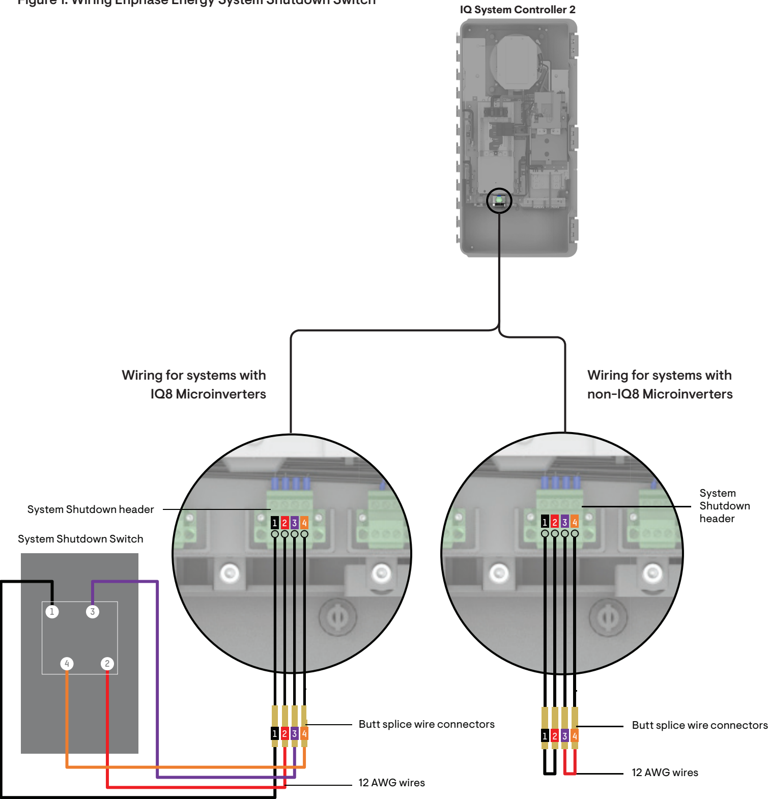
Figure 1: Wiring Enphase Energy System Shutdown Switch
